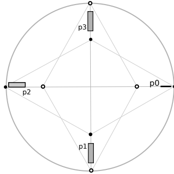
Figure 2.1: The sets defining \Omega .
