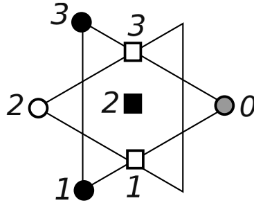
Figure 4.1: Polar and equatorial versions of the TBP.
