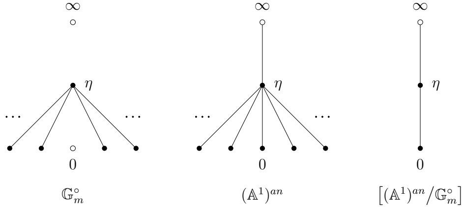
FIGURE 8. Consider the affine line \mathbb{A}^1 over a trivially valued field k . The non-Archimedean unit circle \mathbb{G}_m^\circ is given as the subset of elements in x \in (\mathbb{A}^1)^{an} with |t|_x = 1 , where t denotes a coordinate on \mathbb{A}^1 . The skeleton \mathfrak{S}(\mathbb{A}^1) of (\mathbb{A}^1)^{an} is the line connecting 0 to \infty . It is precisely the set of " \mathbb{G}_m^\circ -invariant" points in (\mathbb{A}^1)^{an} and therefore naturally homeomorphic to the topological space underlying [(\mathbb{A}^1)^{an}/\mathbb{G}_m^\circ] (see [Uli14, Example 6.2]).
