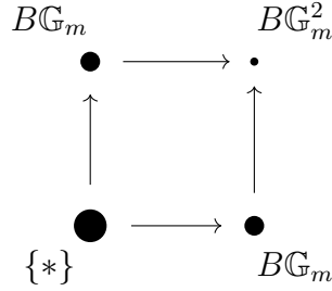
FIGURE 7. \mathcal{A}_{\mathbb{N}^2} . The small closed point is B\mathbb{G}_m^2 , the intermediate points are B\mathbb{G}_m and the big point is just a point.
