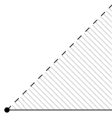
FIGURE 6. The fan of the Whitney umbrella drawn as a cone—the first quadrant—folded over itself via the involution (x, y) \mapsto (y, x) .
