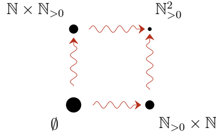
FIGURE 4. Points and topology of \text{Spec } \mathbb{N}^2 . The big point corresponds to the ideal \emptyset , the intermediate points are the primes \mathbb{N} \times \mathbb{N}_{>0} and \mathbb{N}_{>0} \times \mathbb{N} , and the small closed point is the maximal ideal \mathbb{N}_{>0}^2 . The arrow indicate specialization, thus determining the topology.
