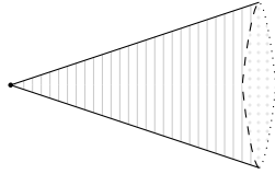
FIGURE 3. The complex of \mathbb{P}^2 with the divisor consisting of a line and a transverse conic: the cones associated to the zero strata meet along both their edges.
