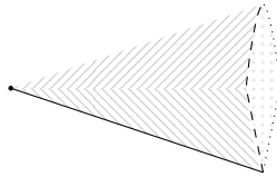
FIGURE 5. The fan of the nodal cubic drawn as a cone with the two edges glued to each other.
