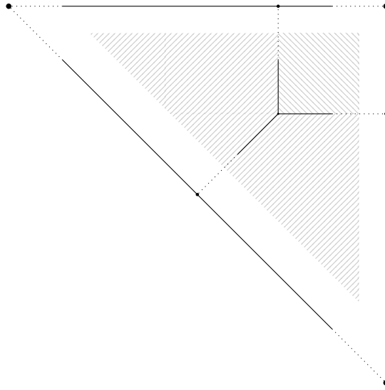
FIGURE 2. The extended fan of \mathbb{P}^2
