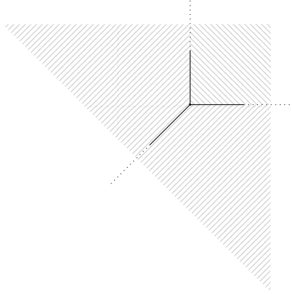
FIGURE 1. The fan of \mathbb{P}^2
