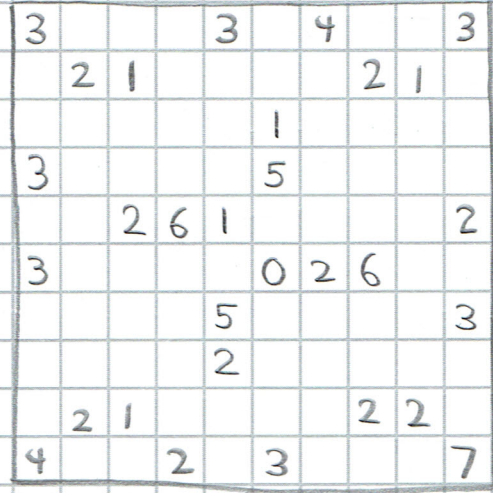
Inside/Outside Sudoku
