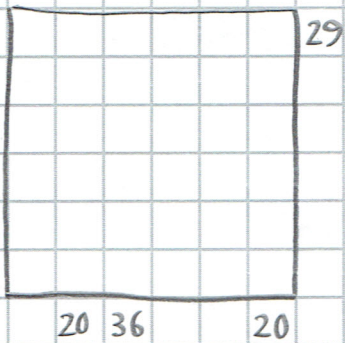
Geometric Distribution
