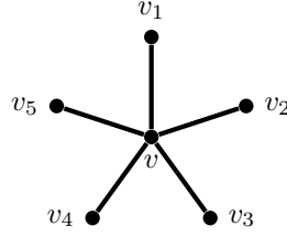
Figure 2.9: A degree 5 vertex v with its 5 neighbors
