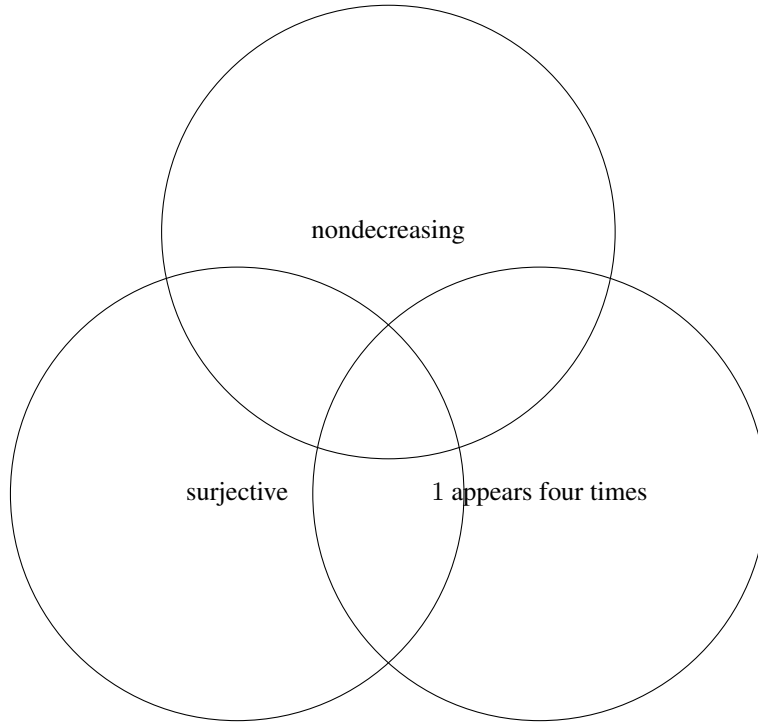
Figure 1.4: Venn diagram of functions [6] \rightarrow [3] for Exercise 1.20.
