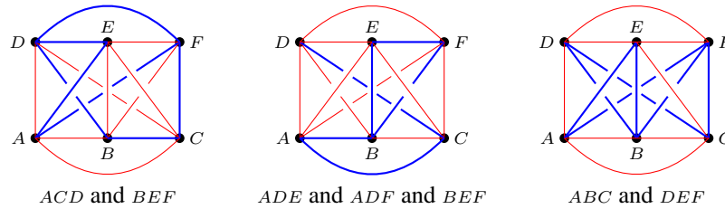
Figure 2.10: Some 2-edge colored K_6 graphs with indicated monochromatic triangles
