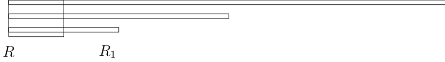
FIGURE 2. The proof that \mathcal{B}_1(\mathcal{B}_1(\mathcal{U})) is empty.
