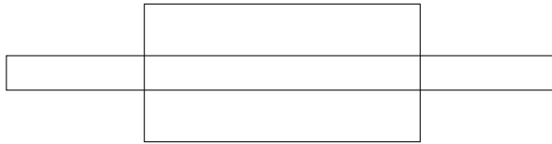
FIGURE 1. Two intersecting rectangles in the plane. The two sides are in inverse relation.
