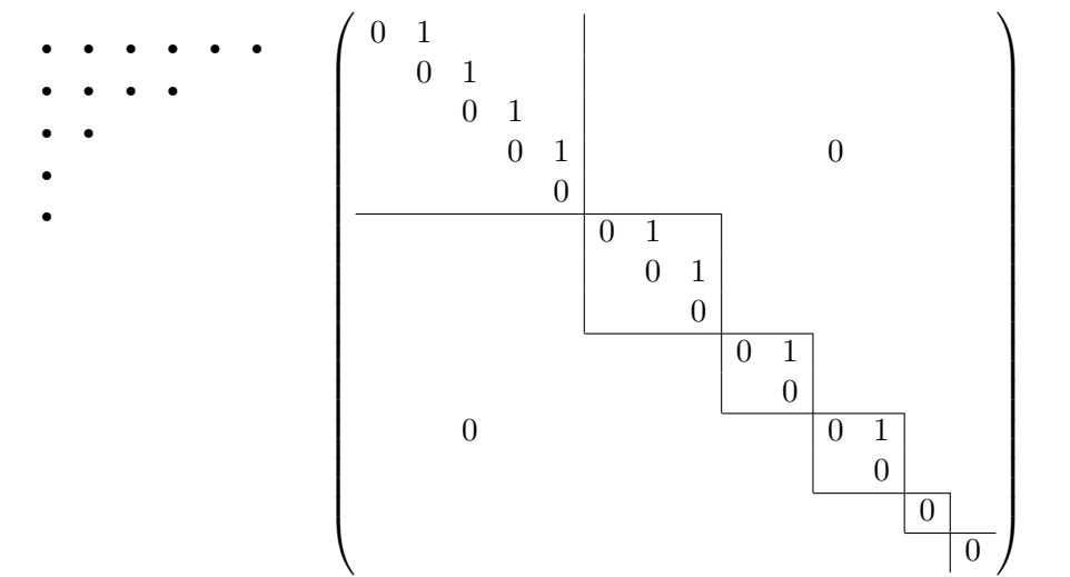
Figure 1. Dot diagram and corresponding Jordan canonical form of a nilpotent operator
